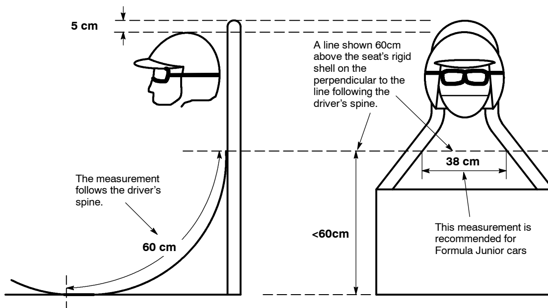
Fig 1. Roll over hoop dimensions [Drawing K62 from Appendix K]
