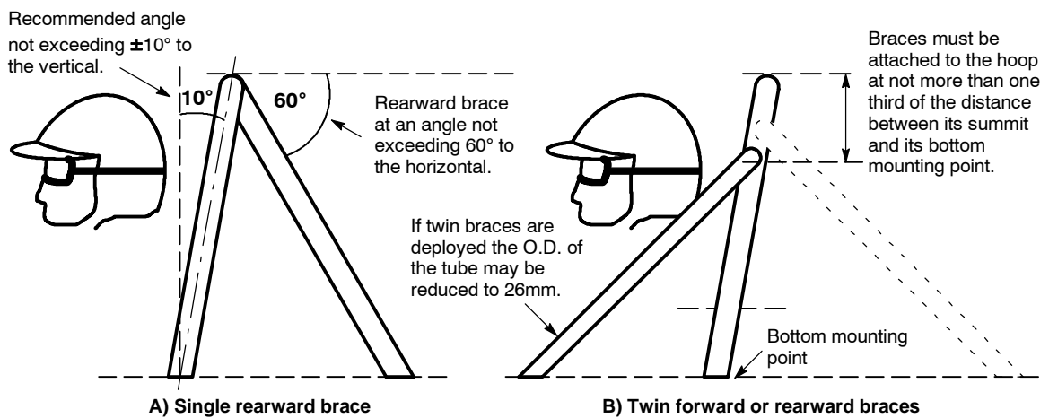
Fig 2. Roll over protection structure bracing guidelines
